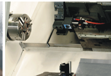
Laser calibration
