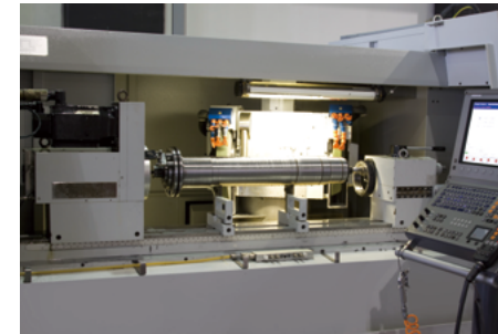
High-precision spindle grinding
