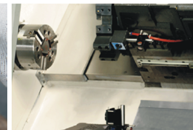
Laser calibration
