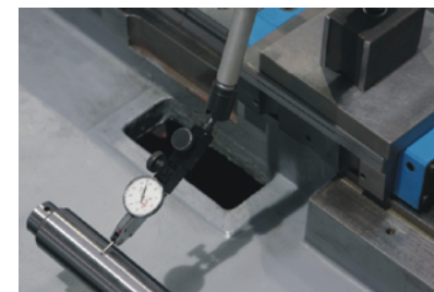
Assembly inspection
